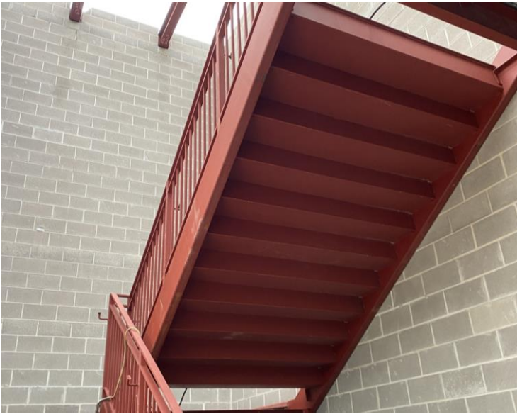
Classroom stair tower and steel framings on SW corner
